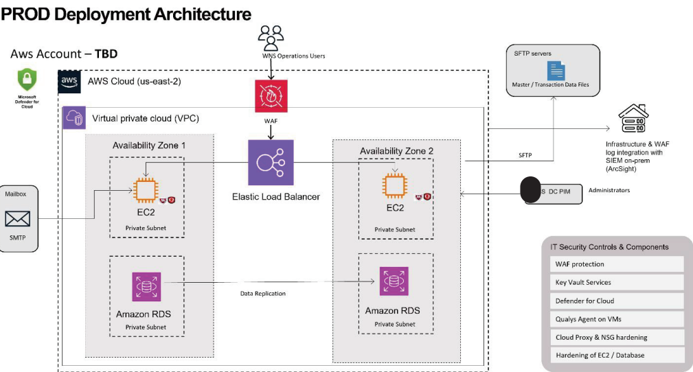
(b) Deployment Architecture
